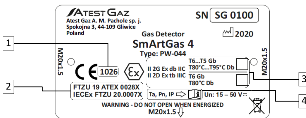
Figure 2: Information on the rating plate of the device
