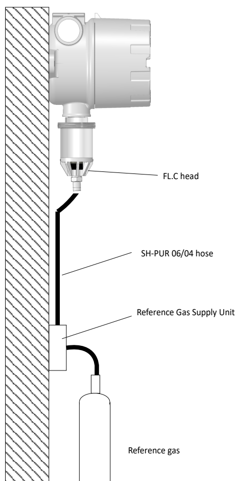
Figure 3: Calibration of a gas detector with the F.L.C head
